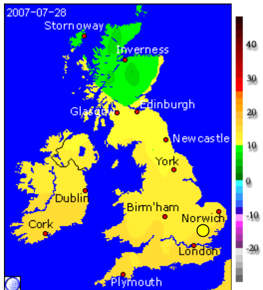
Forecast Min Temperature (°C) Sat 28 Jul
